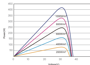
P-V CURVES OF PV MODULE(415W)
