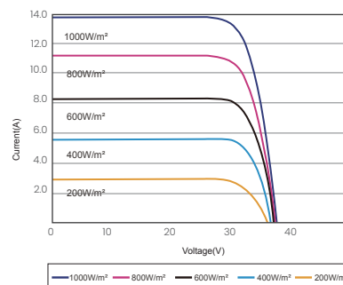
I-V CURVES OF PV MODULE(415W)
